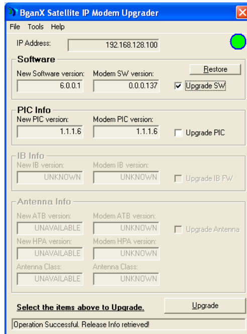
Figure 1: Sample Upgrader Screen while in Normal Mode
