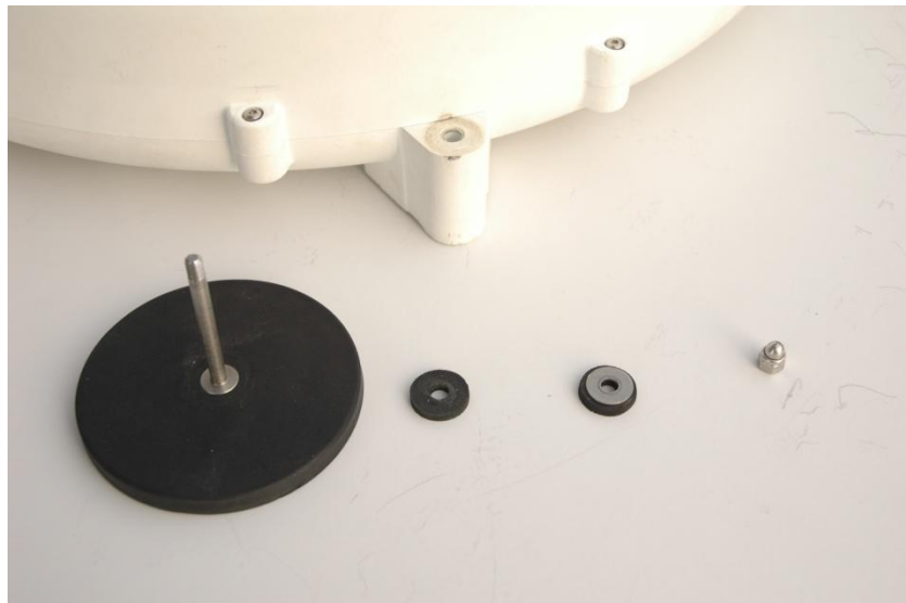
Figure 14 – C10 Antenna with Magnetic Mount Component Parts
