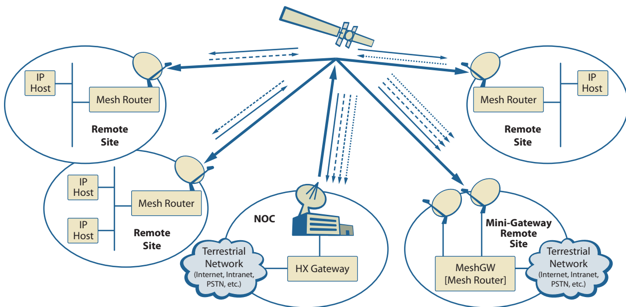
HX System Architecture for Mesh Connectivity
